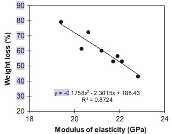
64 Fig. 10 Relationship between weight loss and modulus of elasticity
