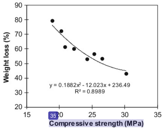
17 Fig. 9 Relationship between weight loss and compressive strength
